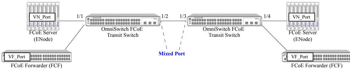
Figure 5-5 : FCoE Port Role-Mixed
